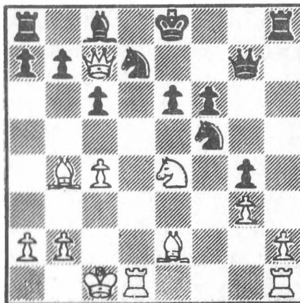
258 After 18...Qg7
